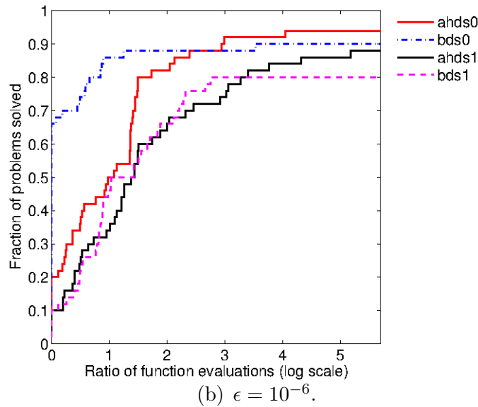
FIGURE 1. Performance of the methods with polling choices 0/1, given a budget of 2000n evaluations.
