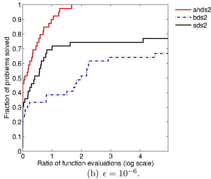
FIGURE 3. Second-, first- and weakly second-order direct-search methods, with polling choice 2 and a budget of 2000n evaluations.
