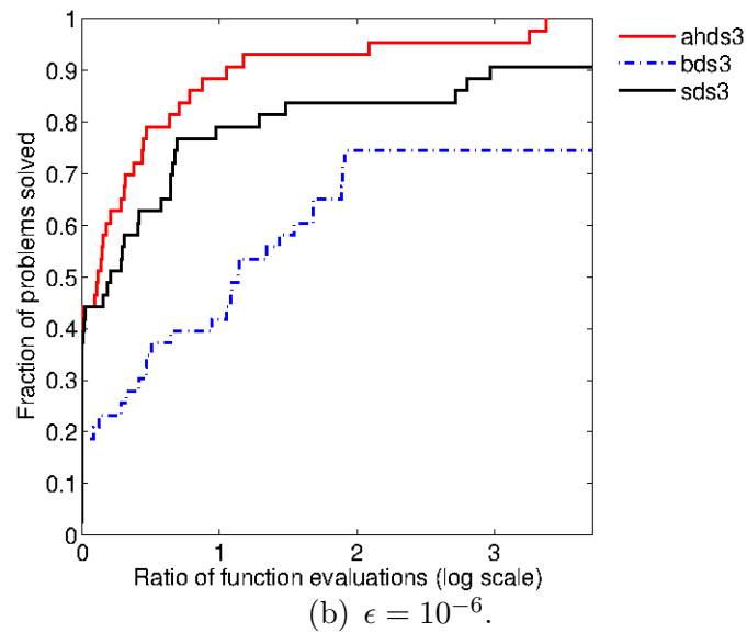
FIGURE 4. Second-, first- and weakly second-order direct-search methods, with polling choice 3 and a budget of 2000n evaluations.
