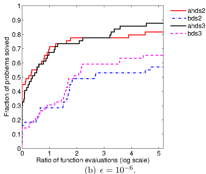
FIGURE 2. Performance of the methods with polling choices 2/3, given a budget of 2000n evaluations.
