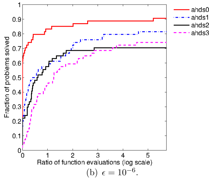
FIGURE 5. Comparison of the ahds methods, given a budget of 2000n evaluations.
